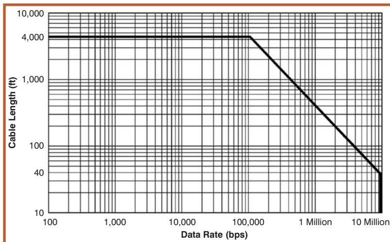
Figure 2: A graph depicting cable length and data rate of RS-485. Source: National Instruments Application Note 1057 “Ten Ways to Bulletproof RS-485 Interfaces.”
