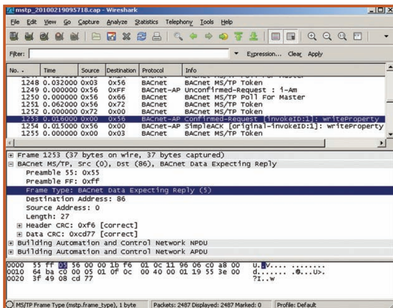
Figure 1: A protocol analyzer displays a BACnet MS/TP frame in all its gory detail.
